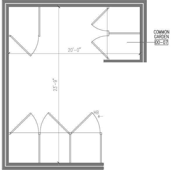
FIRST FLOOR - COMMON GARDEN
